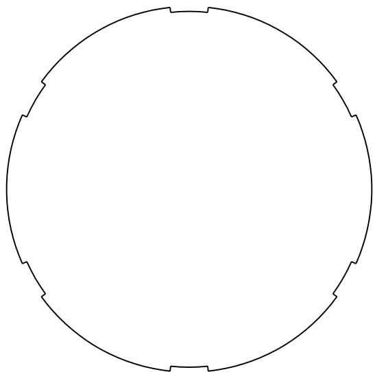
Conventional 6 Groove Rifling
